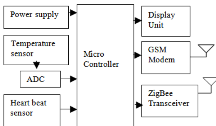
Fig.1 The system architecture at the patient end
